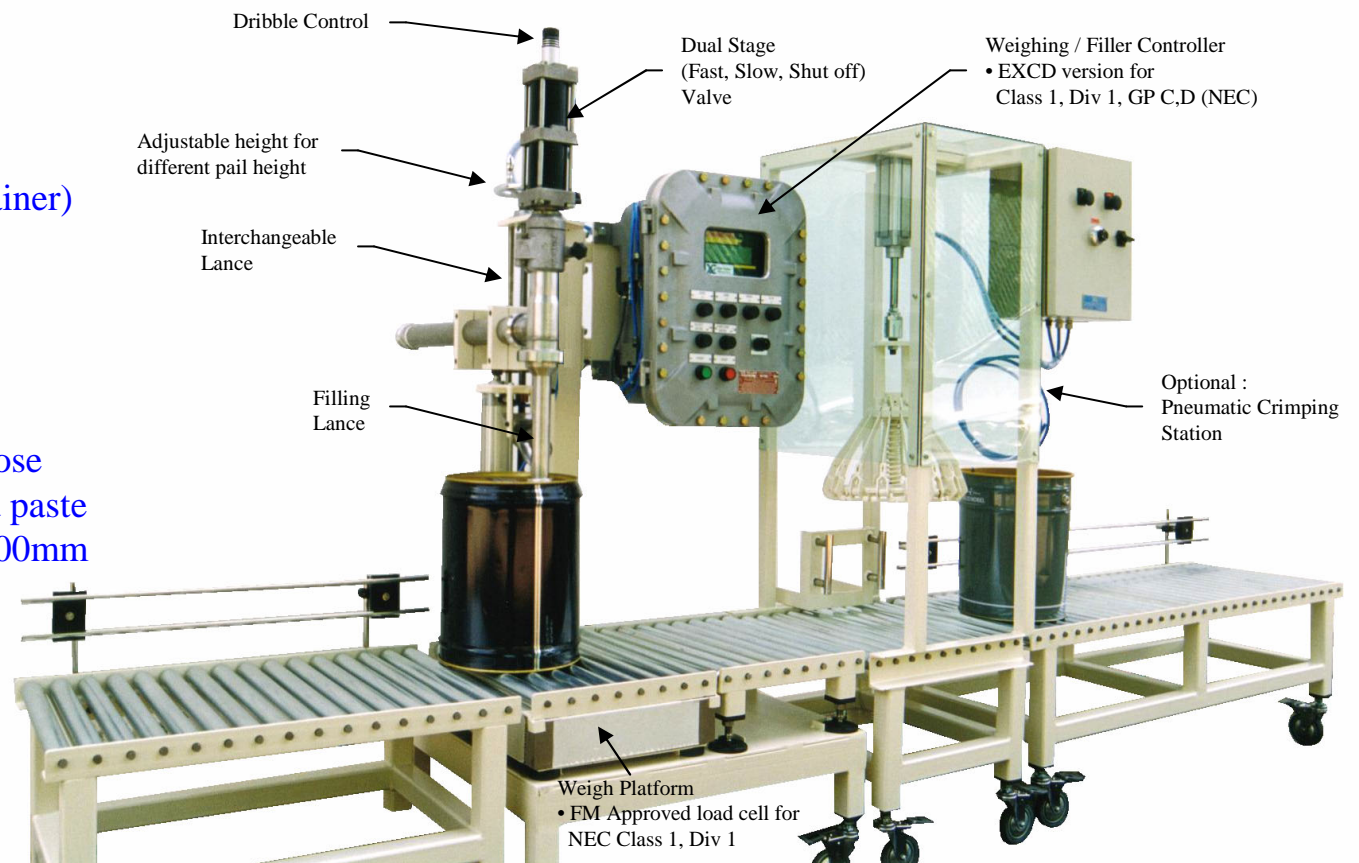
◆ Explosion-Proof Pail Filler c/w pneumatic pail crimper
