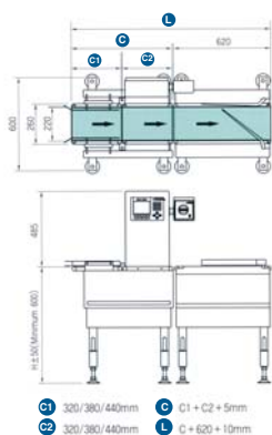
Dimension + Flip Bar Rejector Application (Unit:mm)
