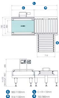
Dimension • Pusher on Roller Rejector (Unit: mm)
