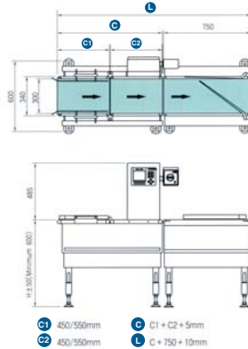
Dimension + Flip Bar Rejector Application (Unit:mm)
