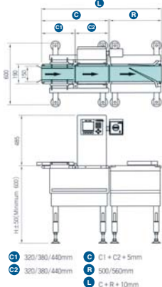
Dimension + Flip Bar Rejector Application (Unit:mm)
