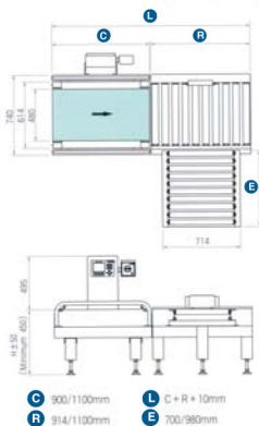
Dimension * Pusher on Roller Rejector [Unit: mm]
